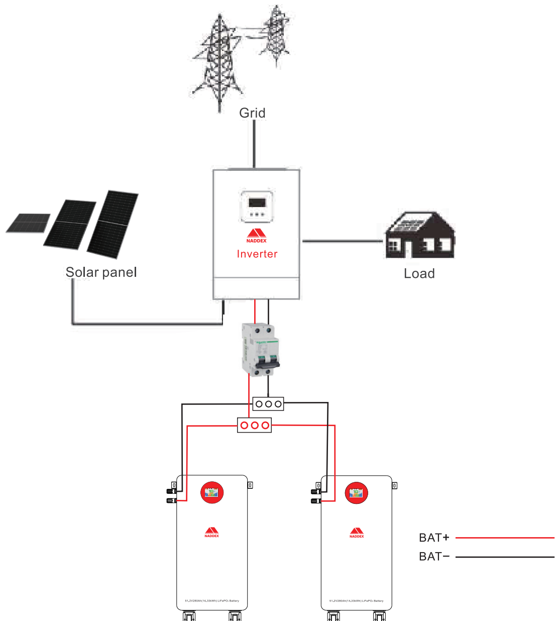
Figure 1 Operation Principle Diagram of Battery System
